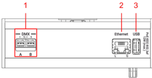
grandMA3 2Port Node DIN-Rail rear panel
