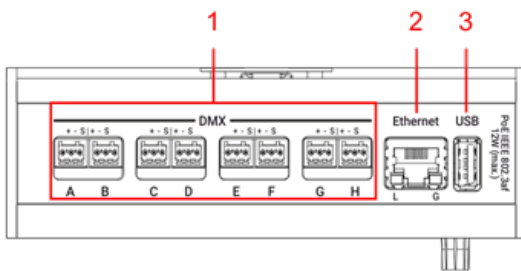
grandMA3 8Port Node DIN-Rail rear panel
