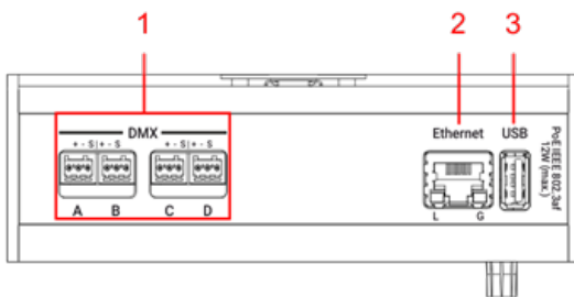
grandMA3 4Port Node DIN-Rail rear panel
