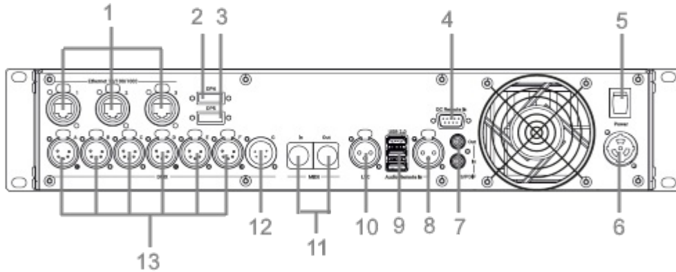
grandMA3 replay unit rear panel
